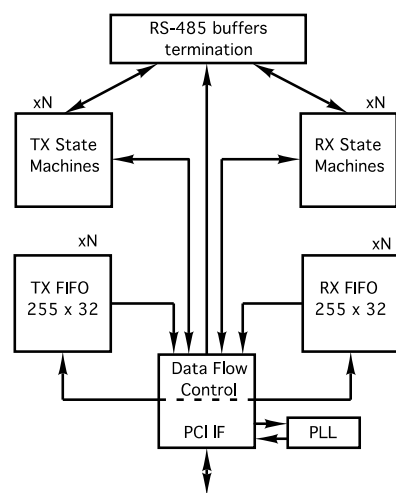
FIGURE 1 PMC-BISERIAL-VI-UART BLOCK DIAGRAM
